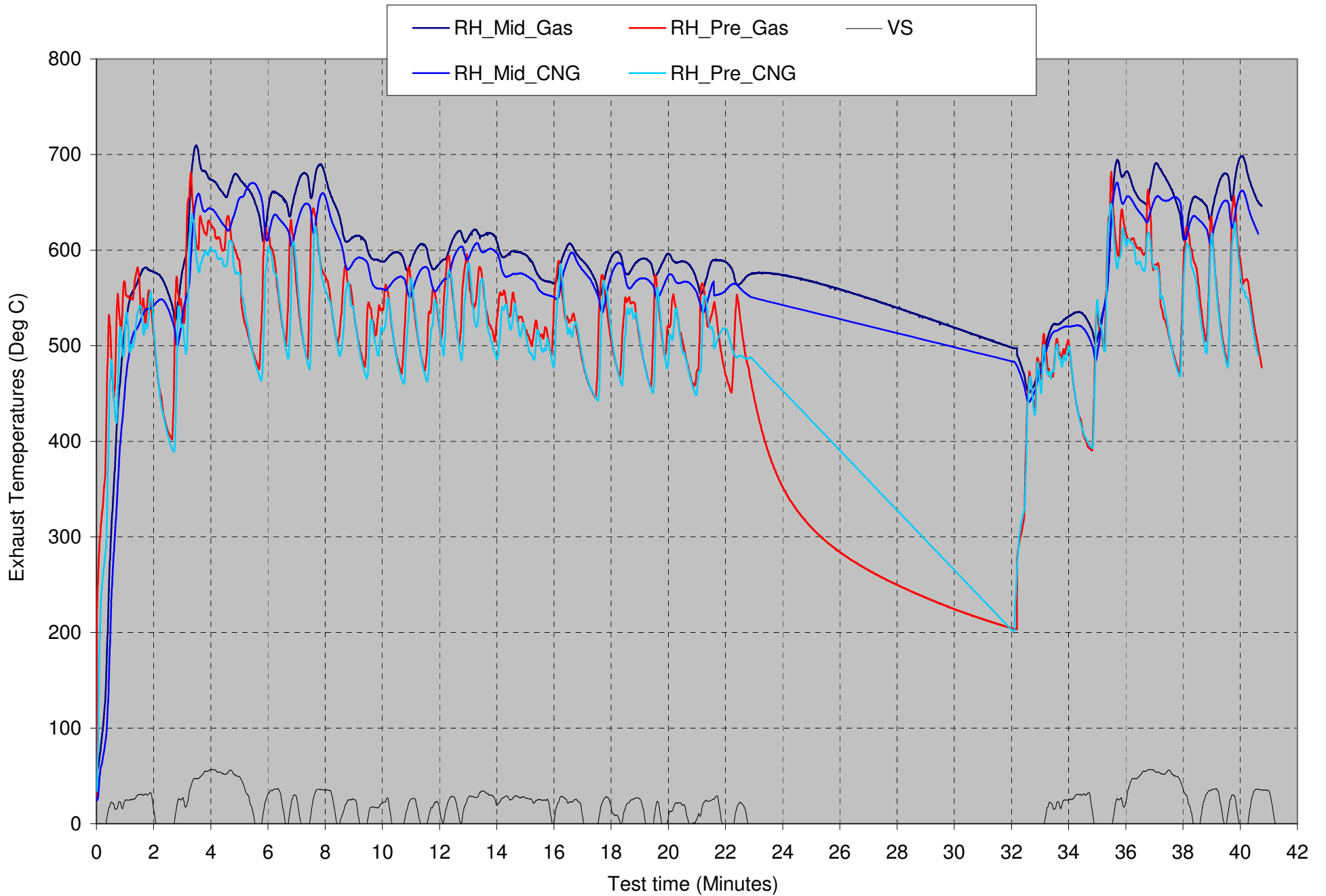
Natural Drive EPA75 Exhaust Temperature Characteristics
